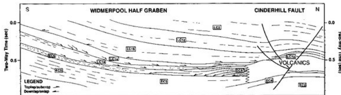
(Figure 12) Sequence architecture, northern margin of the Widmerpool half-graben. LC2 delta top; LC1c delta slope; LC1b prodelta turbidites; LC1a distal prodelta; LC1a' carbonate shelf/condensed mudstone sequence; EC6' carbonate rimmed shelf margin; EC6 basinal carbonates; EC5 basinal mudstone; EC4 basinal carbonate; EC3 basinal carbonate and mudstone; EC2 shelf carbonates; EC1 evaporite/ carbonate slope deposits. Reproduced from Ebdon et al. (1990)
