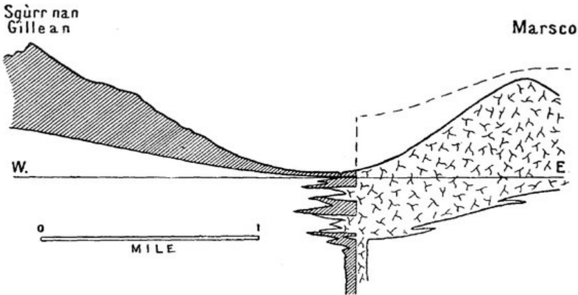
FIG. 26.—Section across Glen Sligachan from Sgùrr nan Gilleán (gabbro) to Marsco (granite), to illustrate the supposed nature of the western boundary of the granite in this part.
