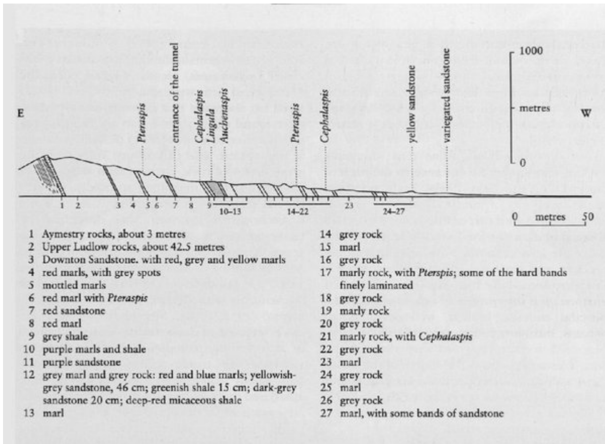
(Figure 3.13) Section at Ledbury railway cutting recorded by Symonds (1860). Even more than 100 years later much of this section was still visible; recently, however, much of the western end has become obscured.
