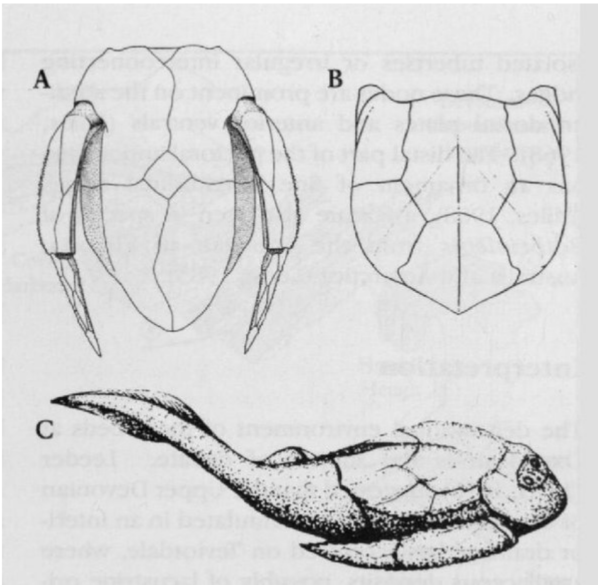
(Figure 8.6) The antiarch Bothriolepis hayi Miles (1968) from the Oxendean Beds of Oxendean Burn. (A) restoration of the trunk-armour in ventral aspect based on RSM 11967.34.43 and FR 1867, x 0.2; (B) restoration of the dorsal trunk armour, somewhat flattened, based on RSM 1967.34.16, x 0.2 (after Miles, 1968); (C) reconstruction of Bothriolepis (after Long, 1995), x 0.42.
