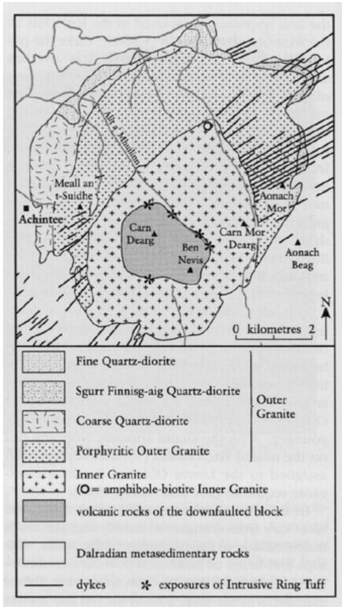
(Figure 9.6) Map showing units comprising the Ben Nevis igneous complex. Note the Inner Granite (essentially a ring intrusion) completely surrounding the down-faulted block. The contact between the two is where the rhyolite and 'flinty crush-rock' (i.e. an ancient vent) is found. The Outer Granite consists of four distinct (and mappable) subunits, emplaced in a margin-to-core sequence. Note also that the dyke-swarm cuts through all subunits of the Outer Granite that lie in its path, but does not penetrate the Inner Granite or the downfaulted block. After Bailey (1960), Burt (1994) and Burt and Brown (1997).
