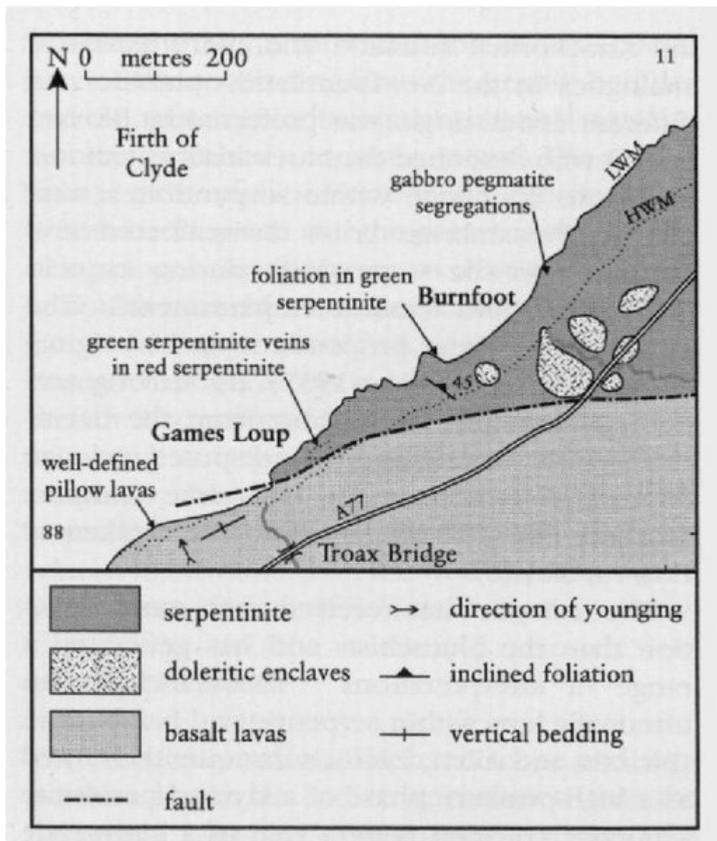
(Figure 2.33) Map of the Games Loup area, after BGS 1:25 000 special sheet, Ballantrae (1988) and unpublished data.
