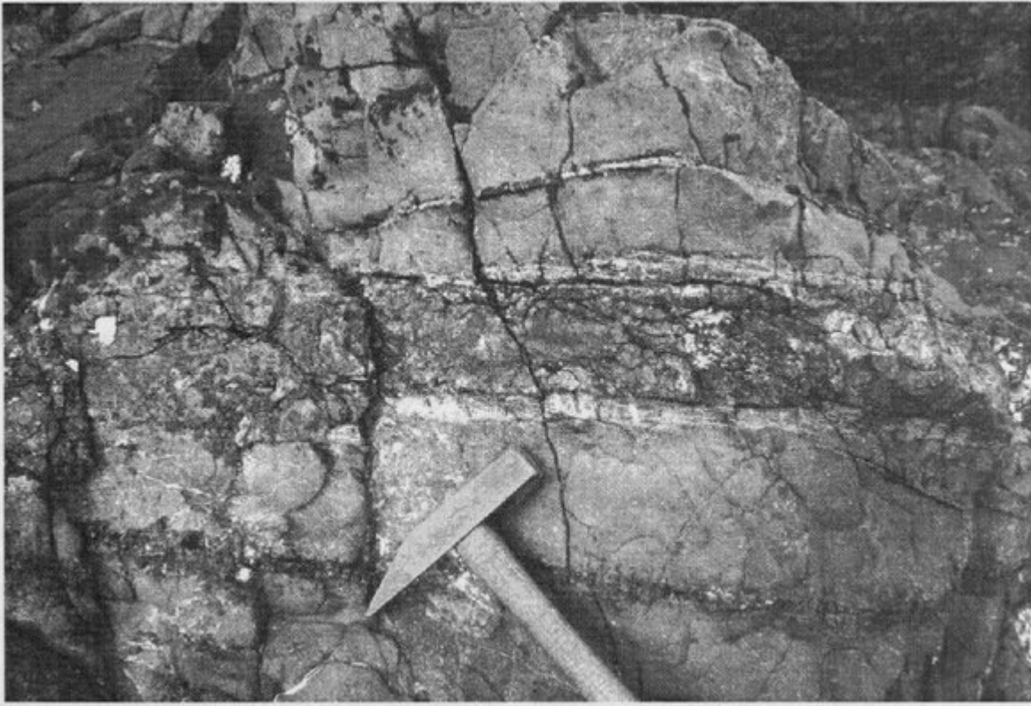
(Figure 2.34) Green serpentinite veins cutting a red serpentinite host at Games Loup. Chrysotile veinlets are developed parallel to the vein margins. (Photo: BGS no. D3345.)
