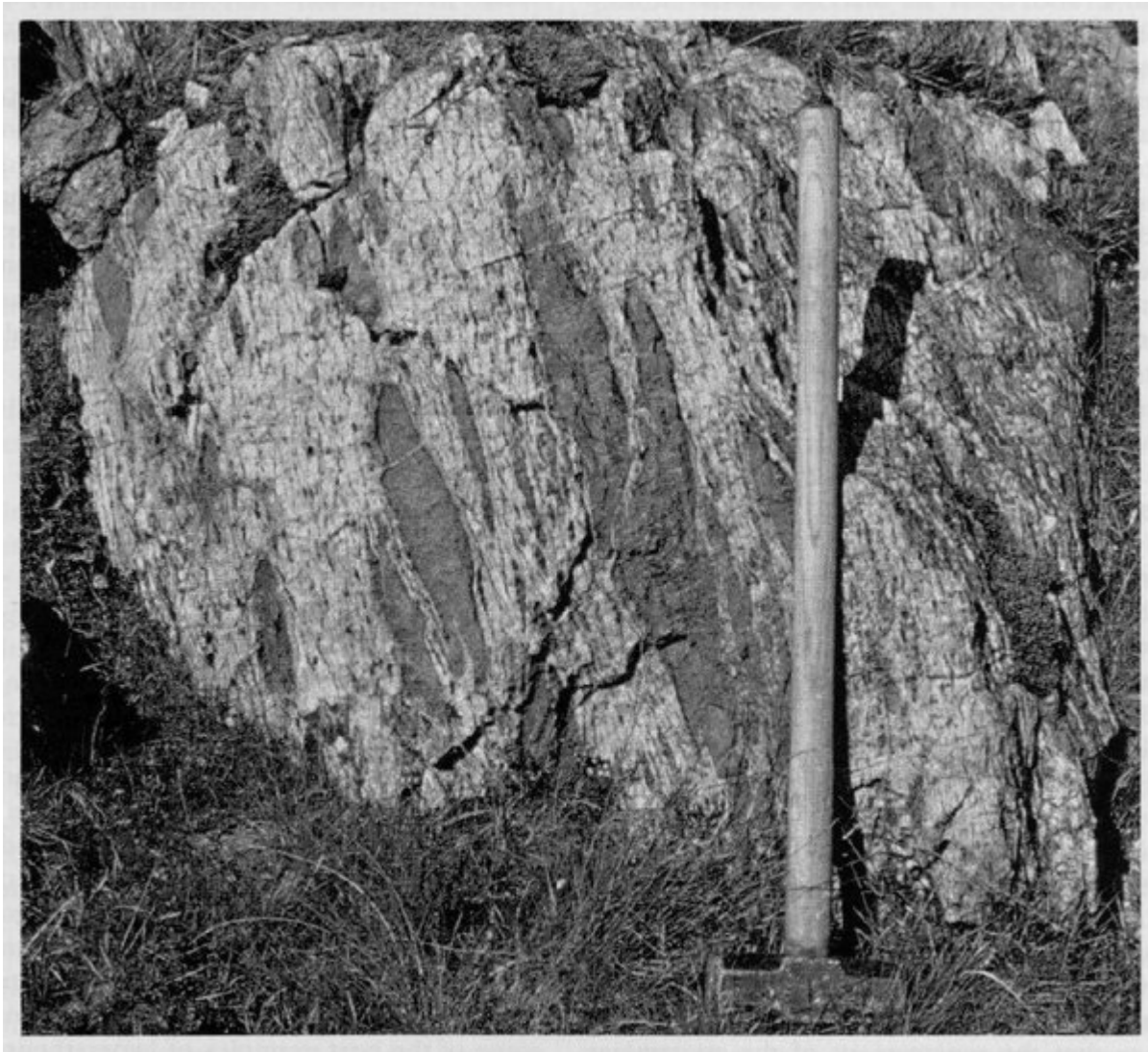
(Figure 8.29) Serpentinized peridotites (wehrlite) at I.ochan Strath Dubh-uisge, Garabal Hill-Glen Fyne igneous complex. (Photo: W.E. Stephens.)
