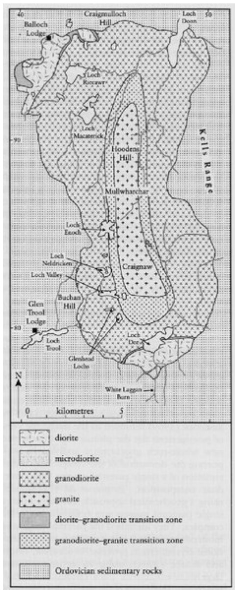
(Figure 8.30) Map of the Loch Doon pluton, based largely on Gardiner and Reynolds (1932) with modifications from Ruddock (1969).
