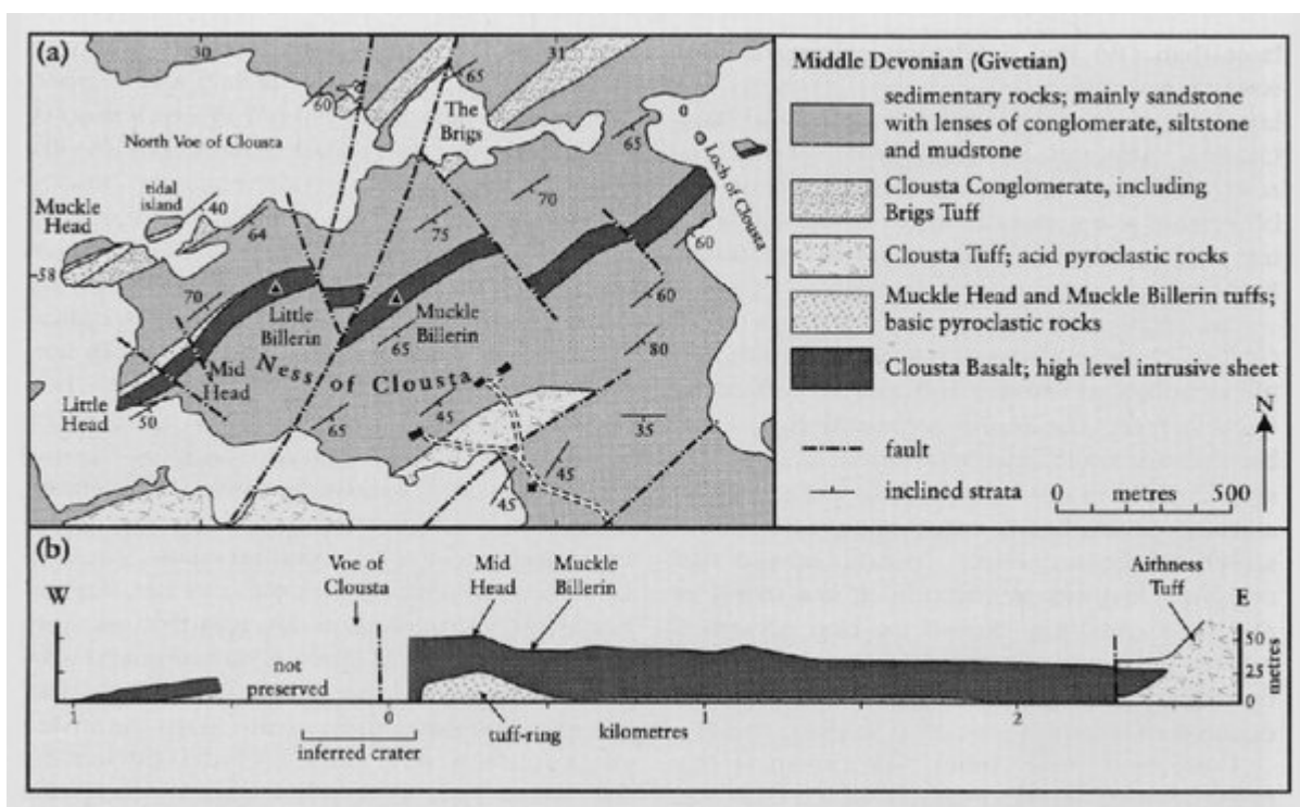
(Figure 9.46) Location of Middle Old Red Sandstone volcanic rocks, major intrusions and major faults in western Shetland, after Mykura (1976).
