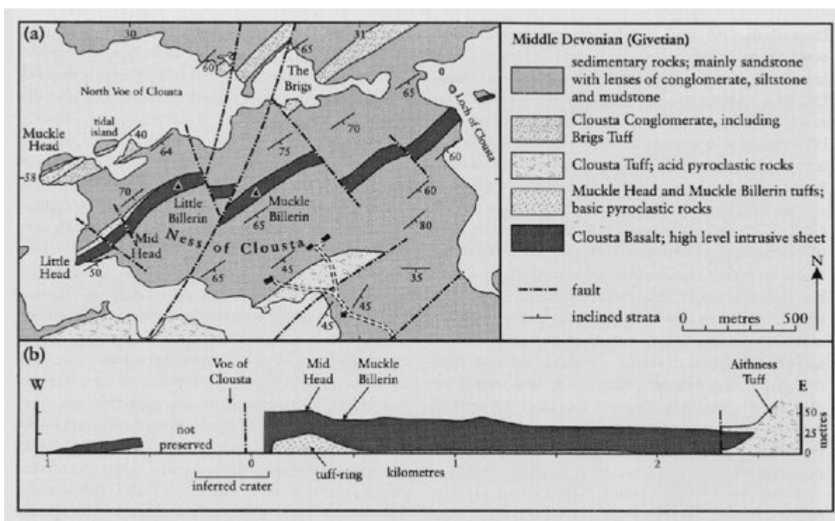
(Figure 9.46) Location of Middle Old Red Sandstone volcanic rocks, major intrusions and major faults in western Shetland, after Mykura (1976).
