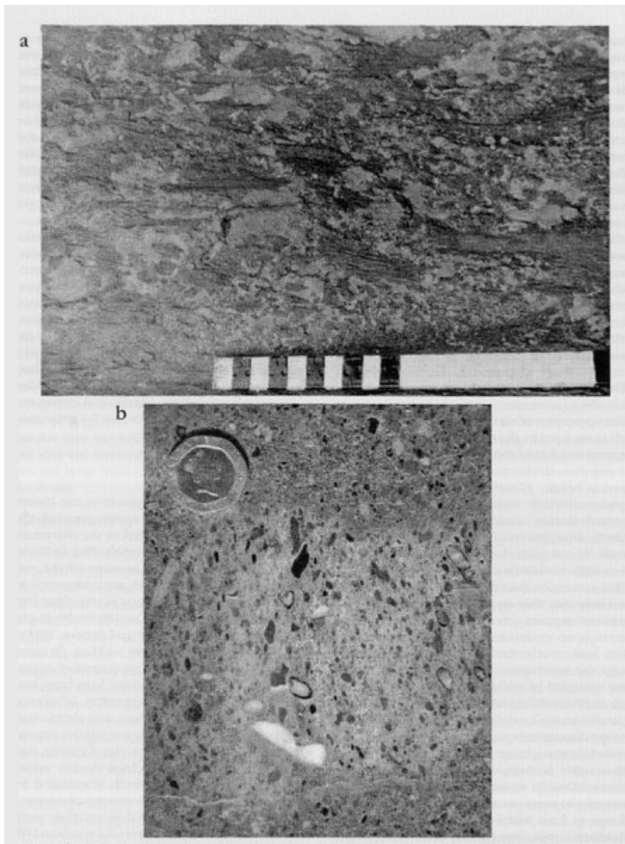
(Figure 4.28) Details of peperitic andesite intrusions in the Seathwaite Fell Formation at Pets Quarry, Kirkstone Pass. (a) Andesite blocks have intruded lacustrine volcaniclastic sands and silts (pale coloured); patches of angular hydroclasts surround some block margins and sediment has been injected into cracks between the blocks. (b) Breccia formed by reworking of hot peperite on the lake floor. Geopetal sand partially infills vesicles later filled with carbonate (white) and chlorite (black) in the large andesite block. White carbonate beneath the block preserves a cavity that probably formed when the hot block heated water in the sediment matrix after its emplacement in a debris flow. The coin is 22 mm across. (Photos: M. J. Branney.)
