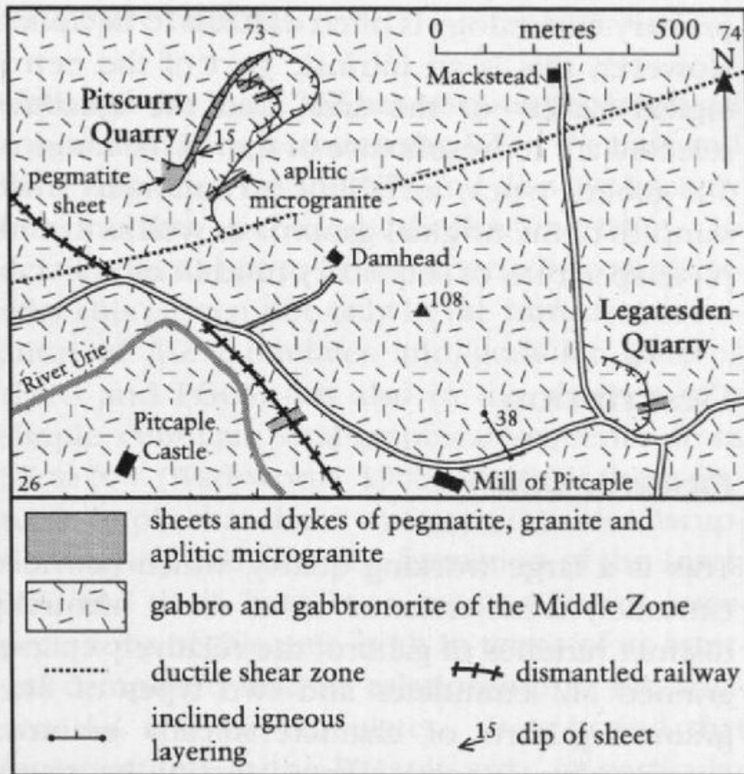
(Figure 3.9) Map of the area around Legatesden and Pitscurry quarries, Insch intrusion, from BGS 1:10 000 Sheet NJ72NW (1989).
