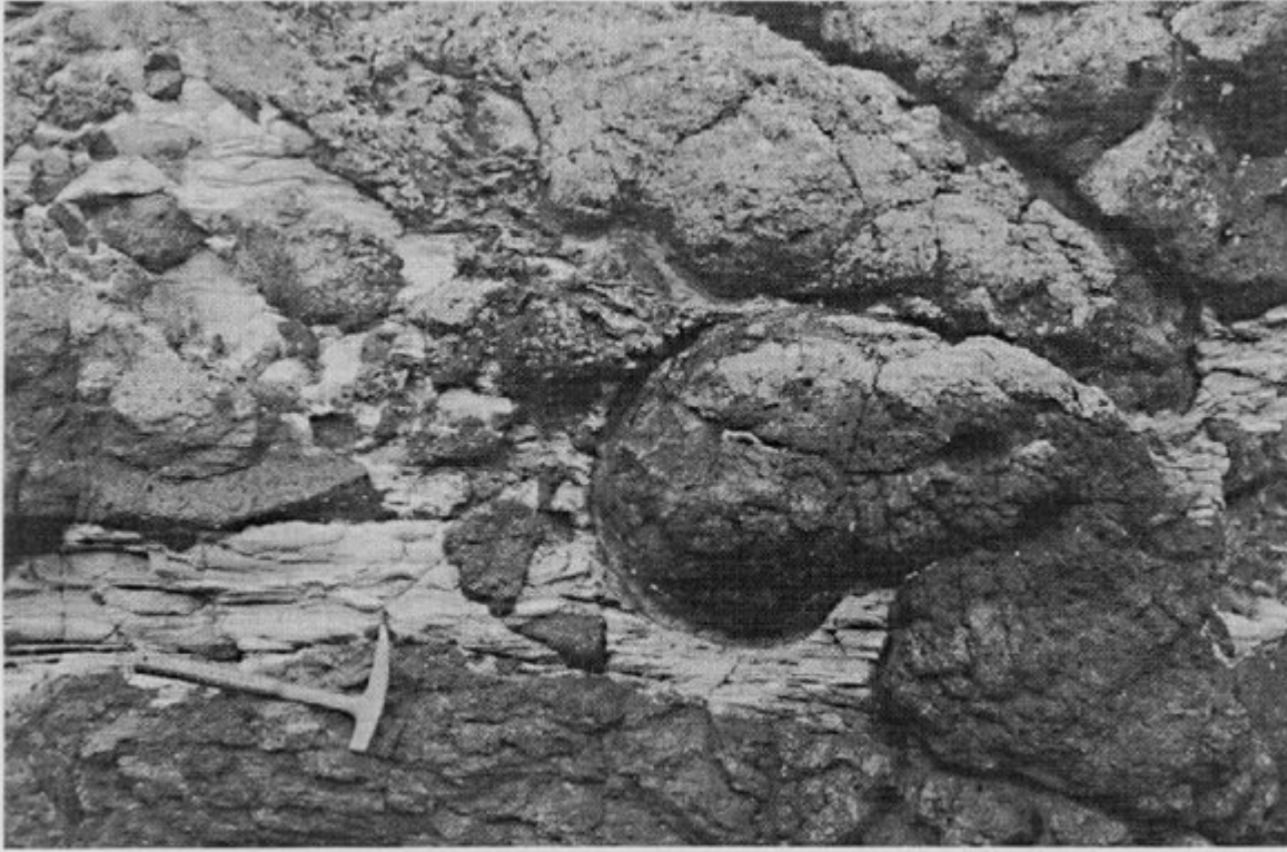
(Figure 9.35) Pillowed lobe of vesicular andesite in laminated sandstone at the base of the south-easterly of the Two Sisters stacks, Port Schuchan [NS 2468 1523]. (Photo: G. Durant.)
