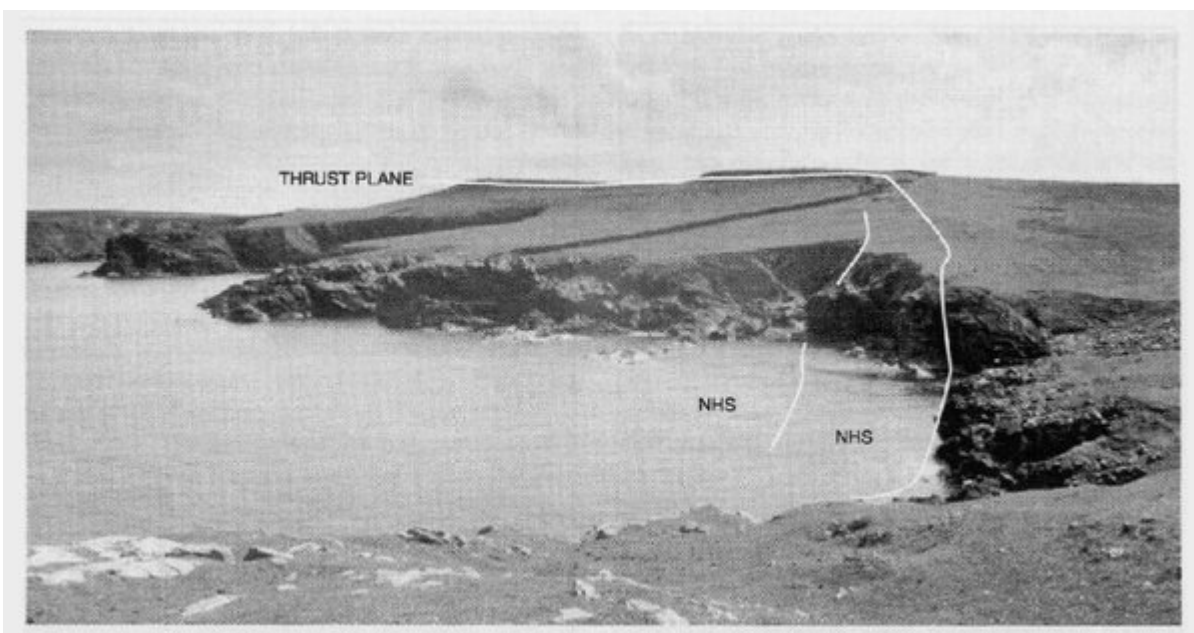
(Figure 2.17) Virva from the north, showing the outcrop of the thrust below the Upper Nappe and the underlying hornblende rocks. NHS, Norwick Hornblende Schist (Photo: D. Flinn.)
