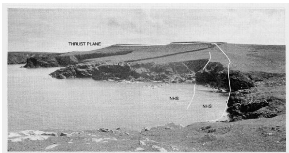
(Figure 2.17) Virva from the north, showing the outcrop of the thrust below the Upper Nappe and the underlying homblendic rocks. NHS, Norwick Hornblende Schist (Photo: D. Flinn.)
