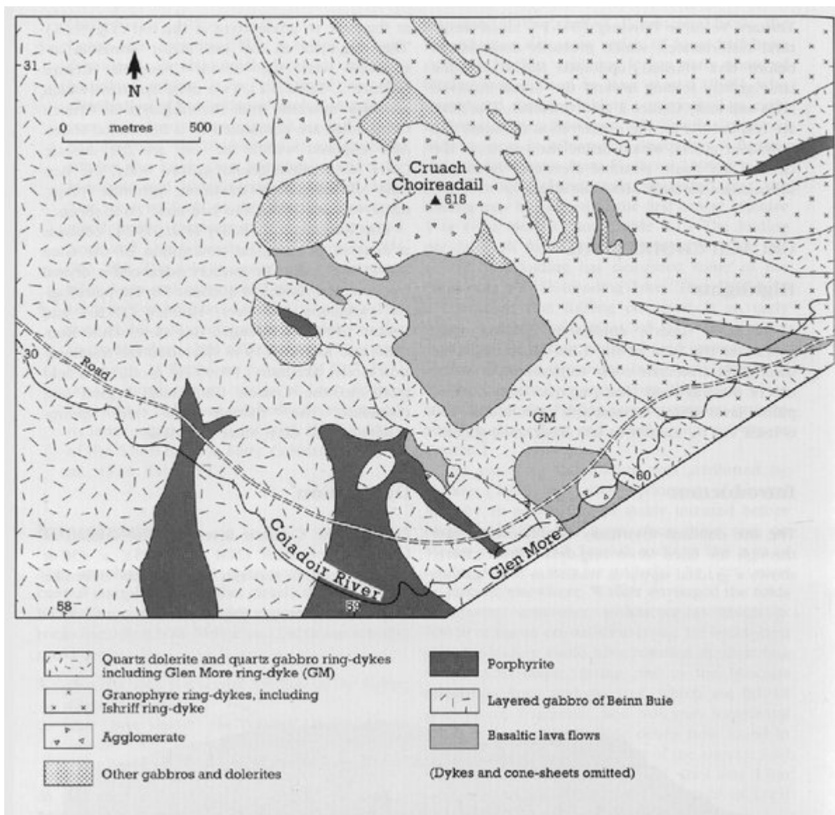
(Figure 5.16) Geological map of the Cruach Choireadail site (adapted from the British Geological Survey 'One Inch' map, Sheet 44, Mull).
