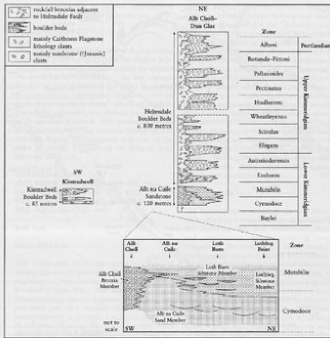
Figure 5.10 Schematic sections showing the main stratal units of the Helmsdale GCR site (based on Macdonald and Trewin, 1993, fig. 2 and Wignall and Pickering, 1993, fig. 15).
