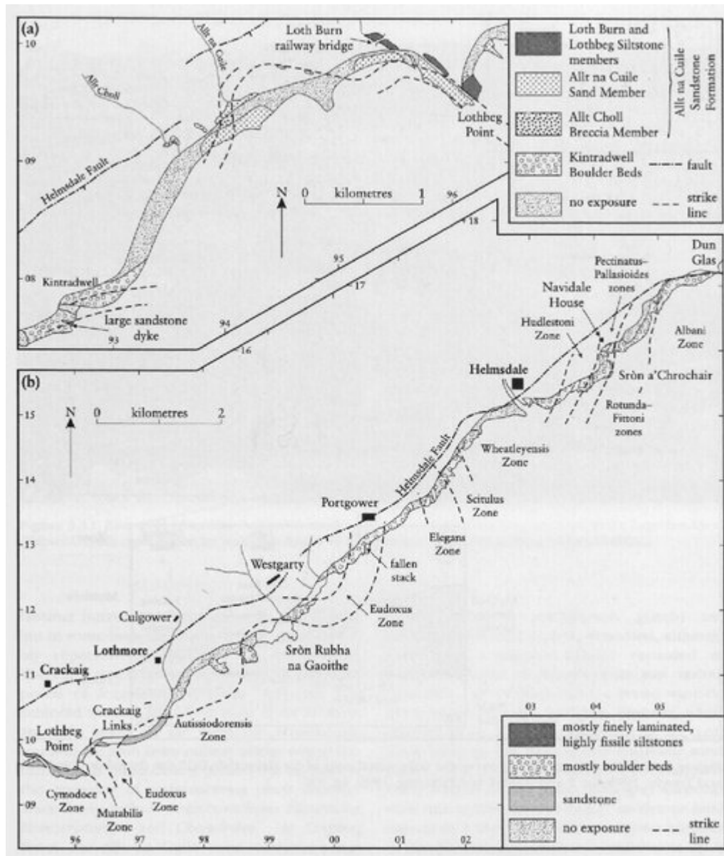
(Figure 5.9) Sketch map of the mainly Kimmeridgian outcrop between (a) Kintradwell and Lothbeg Point, and (b) Lothbeg Point and Dun Glas (after Wignall and Pickering, 1993, figs 10 and 17).
