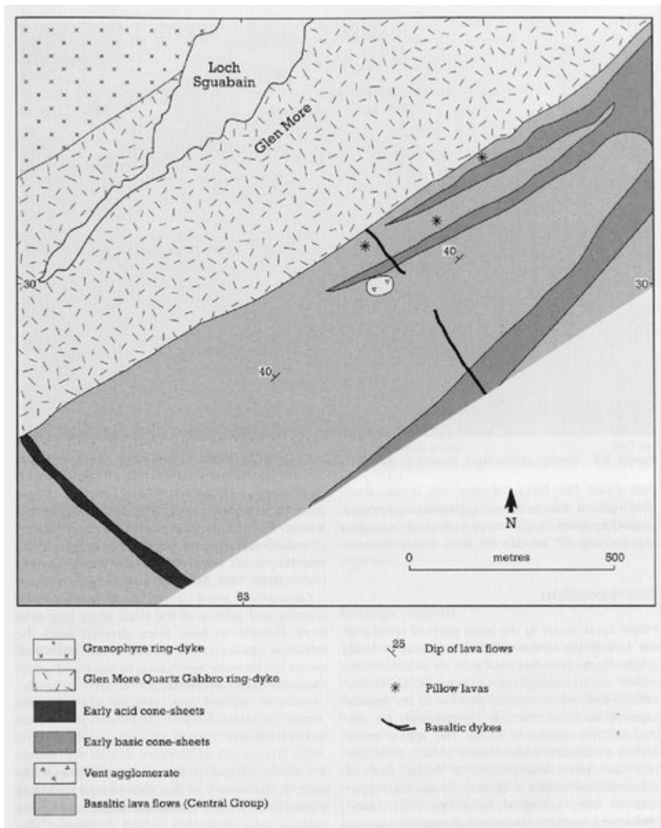
(Figure 5.8) Geological map of the Loch Sguahain site (adapted from the British Geological Survey 'One Inch' map, Sheet 44, Mull).
