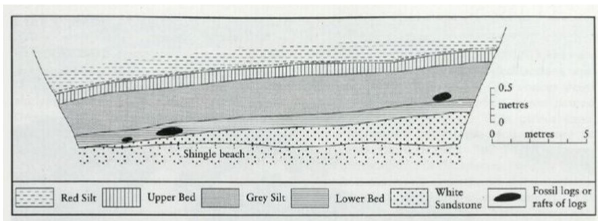
(Figure 6.12) Diagrammatic representation of the two Pseudofrenelopsis Beds at Hanover Point. (After Alvin et al., 1981.)
