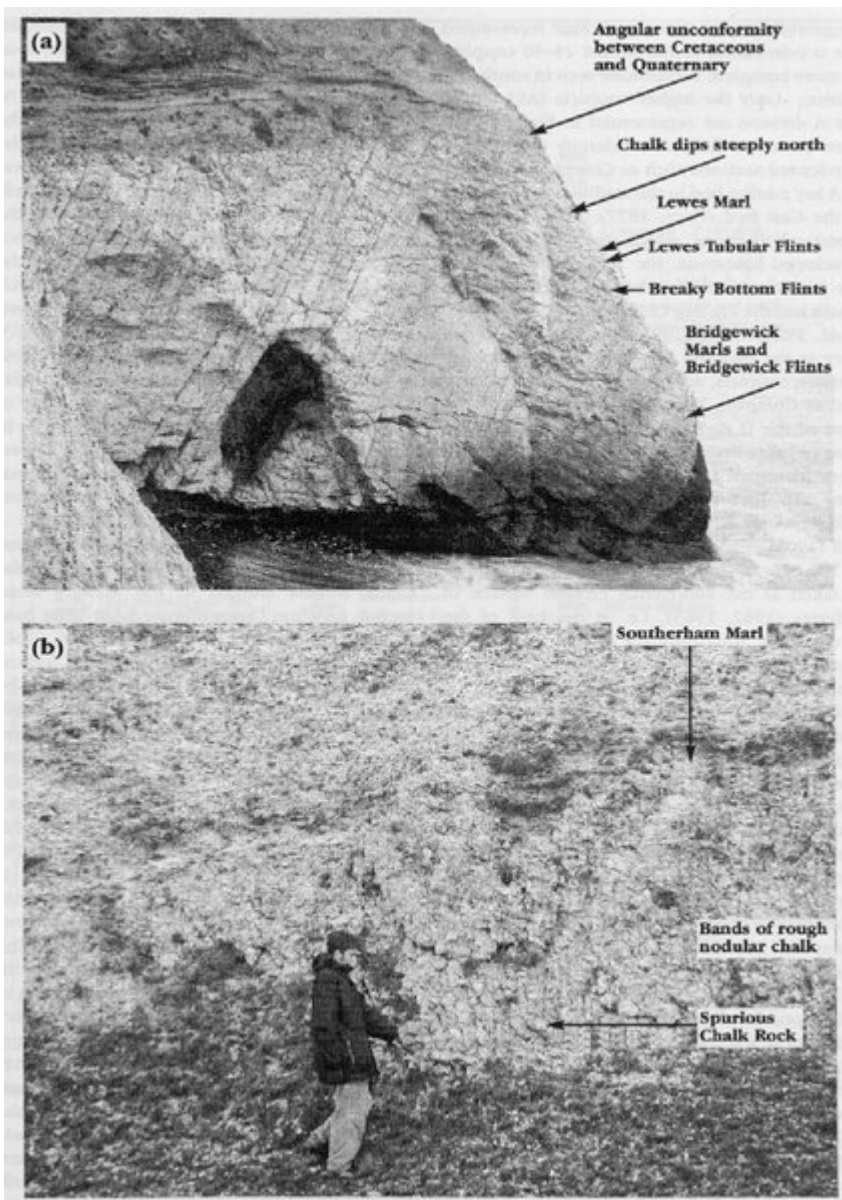
(Figure 3.62) (a) Turanian–Coniacian Lewes Nodular Chalk Formation at the western end of the Compton Bay GCR site, adjacent to Freshwater Bay, Isle of Wight. (b) Base of the Lewes Nodular Chalk Formation in the Compton Down Military Road section in the Compton Bay GCR site, Isle of Wight. (Photos: R.N. Mortimore.)
