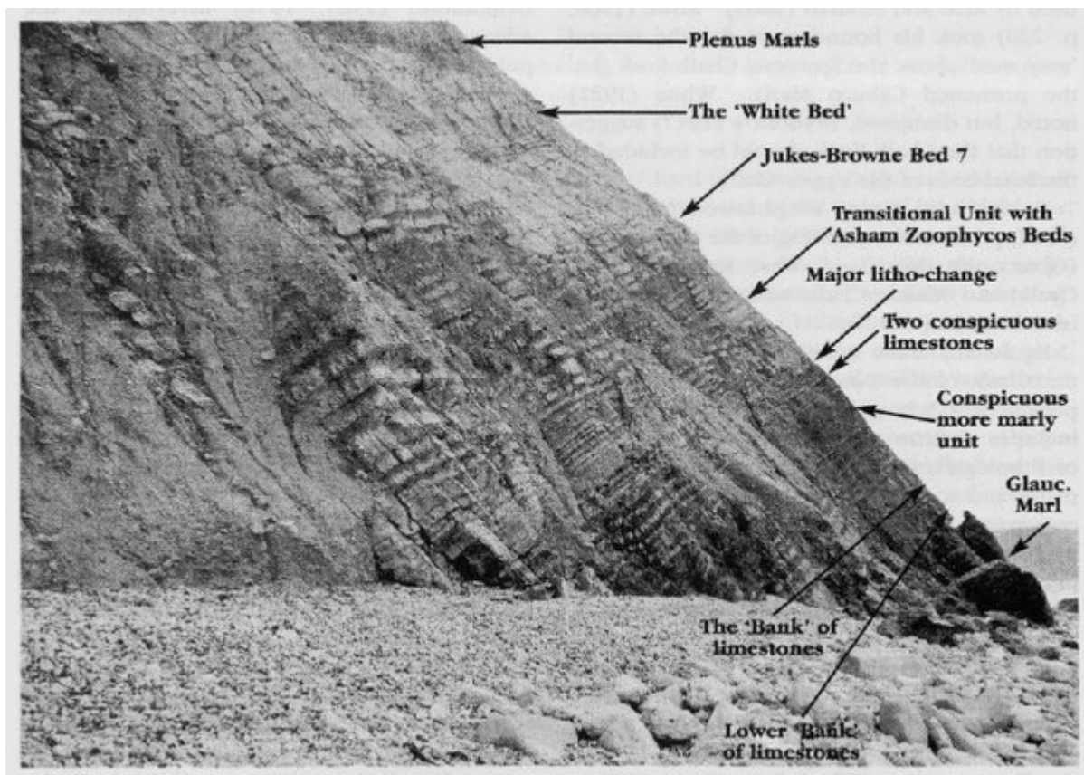
(Figure 3.59) Marker beds in the Cenomanian Grey Chalk Subgroup at Compton Bay, Isle of Wight. Note the conspicuous cyclostratigraphy picked out by marl-limestone couplets. (Photo: R.N. Mortimore.)
