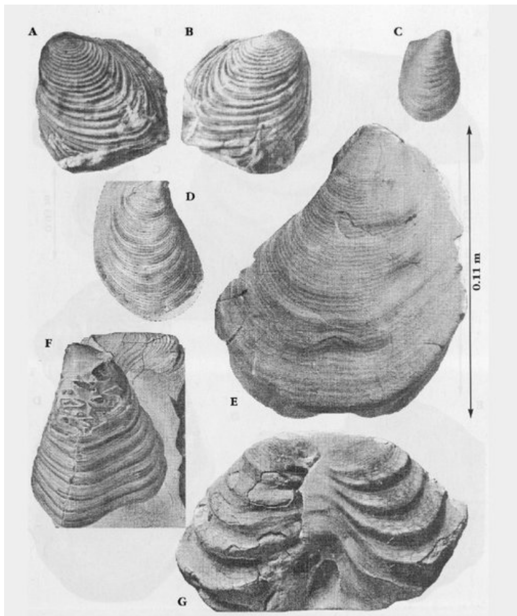
(Figure 2.16) Middle Turonian inoceramid bivalves. (A, B) Mytiloides subbercytticus , typical of the lowest New Pit Chalk (from Seitz, 1934, pl. 40). (C) Inoceramus apicalis (lectotype, from Woods, 1912, pl. 53, fig. 4a), Holywell Nodular Chalk, Hitchin. (D, E) Inoceramus cuvieri ; (D) typical of cuvieri (from Woods, 1912, pl. 53, fig. 7), New Pit Chalk, Royston; (E) the holotype of cuvieri (from Woods, 1912, holotype, text-fig. 73), New Pit Chalk, Royston. (F, G) Inoceramus lamarcki ; (F) the holotype of lamarcki from the Glynde Marls–Southerham Marls interval, Dover (Woods, 1912, text-fig. 63); (G) form typical of mid-New Pit Chalk around Lewes (Woods, 1912, text-fig. 69). Scale bar applies to all specimens.
