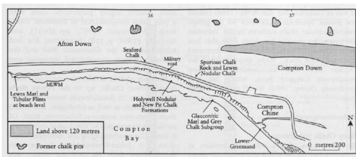
(Figure 3.58) Map showing the details of the Compton Bay site. (MLWM = mean low water mark.)
