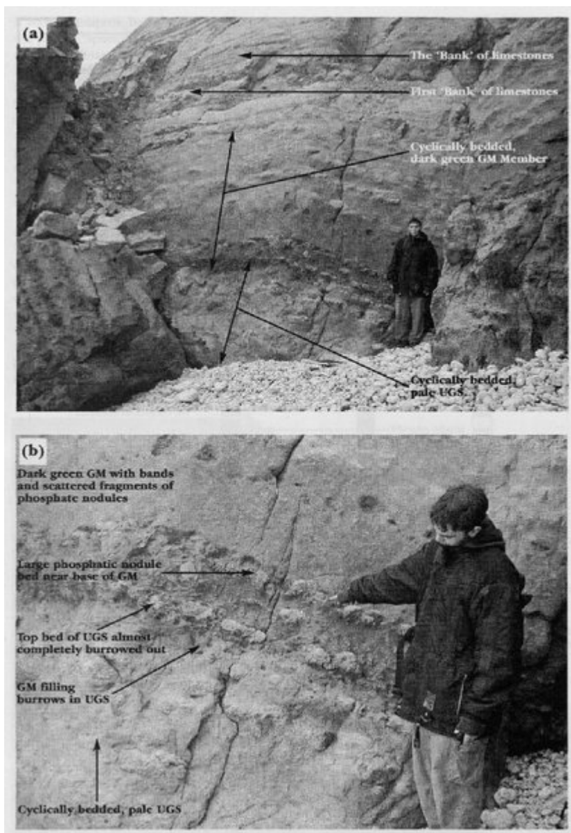
(Figure 3.61) (a, b) The base of the Upper Cretaceous in Compton Bay, Isle of Wight, at the contact between the Albian Upper Greensand and the Cenomanian Glauconitic Marl. (Scale: Tom Mortimore = 1.8 m tall). (GM = Glauconitic Marl; UGS = Upper Greensand). (Photos: R.N. Mortimore.)
