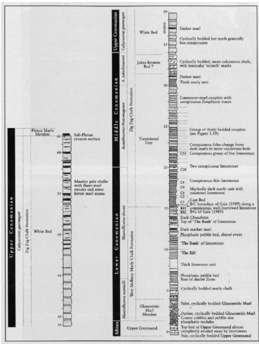
(Figure 3.60) The Grey Chalk Subgroup successions, exposed at Compton Bay, Isle of Wight.
