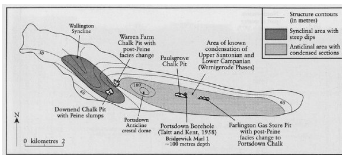
(Figure 3.79) Structure contours on the Chalk of Portsdown, showing the shape of the Portsdown Anticline and Wallington Syncline. Peine phase tecto-sedimentary structures are present at Downend Chalk Pit and Warren Farm
