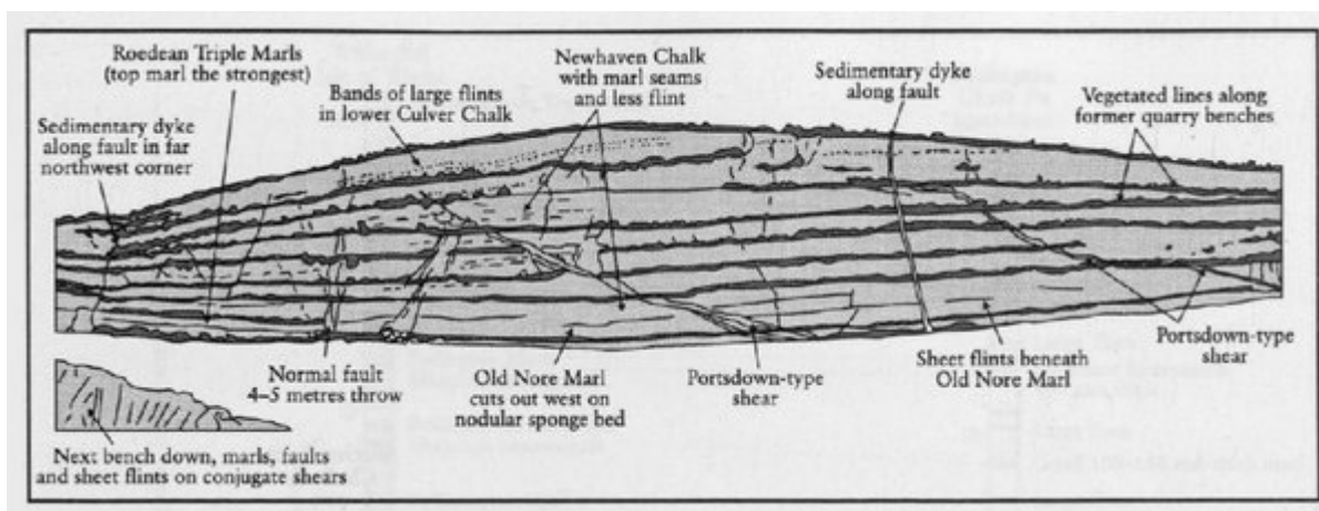
(Figure 3.82) Paulsgrove Chalk Pit, Portsdown, Portsmouth, Hampshire.
