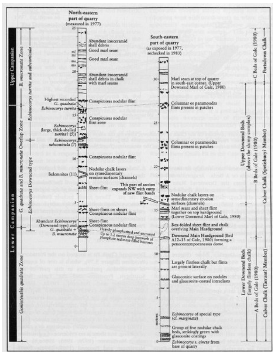
(Figure 3.78) Stratigraphy of the Campanian Chalk originally exposed at Downend Chalk Pit, Portsdown. Any two sections are different as syndimentary channels and growth of penecontemporaneous slump folds create local pockets of expanded or condensed sediments. The sections shown are an attempt to illustrate the total range of the stratigraphy and the main subdivisions unravelled from the slump complex. (ms = marl seam; ml = marly laminae.)
