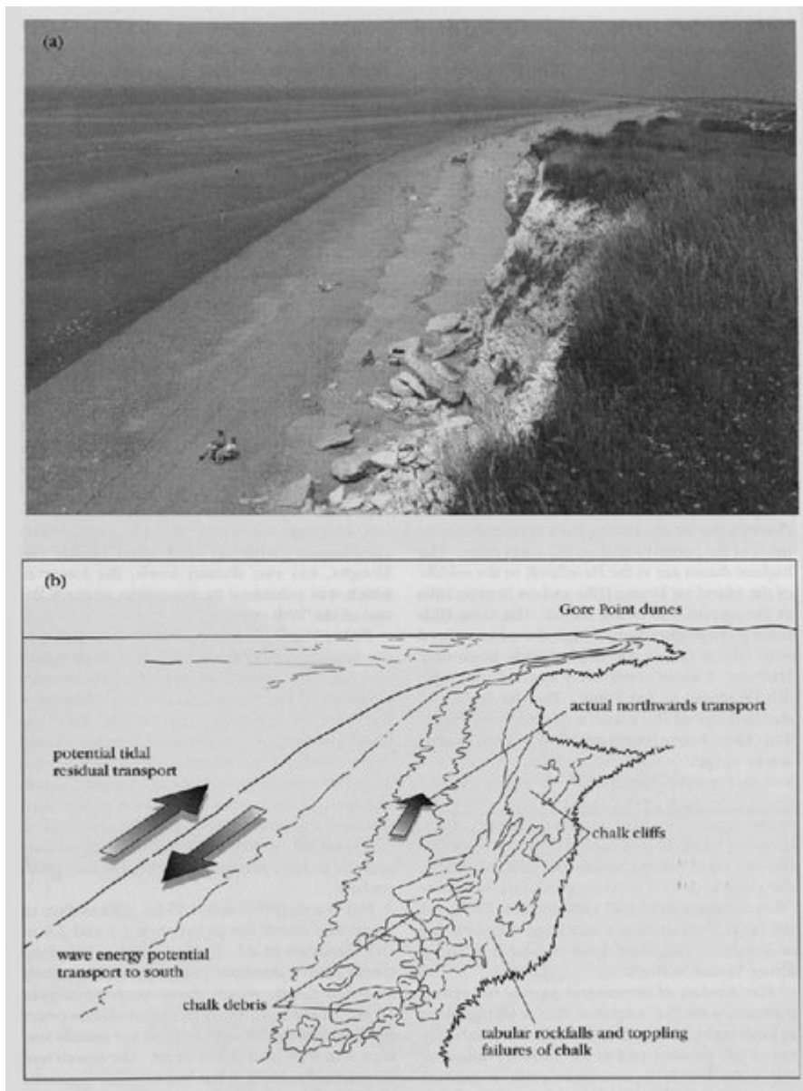
(Figure 11.28) (a) The distinctive tabular chalk cliffs of Hunstanton, looking north. (b) Cartoon of potential transport mechanisms of rockfall debris from the failure of the chalk cliffs. (Photo: V.J. May.)
