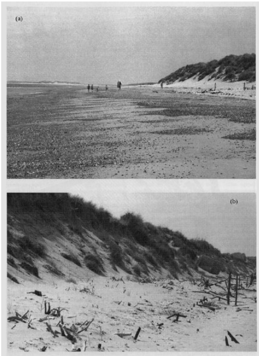
(Figure 11.29) (a) Brancaster beach-dunes, sand and shingle beach with regular shore-normal cusps. (b) Eroded dune-face remnants of World War II defence structures and associated retreating foredune scarp. (Photos: V.J. May.)
