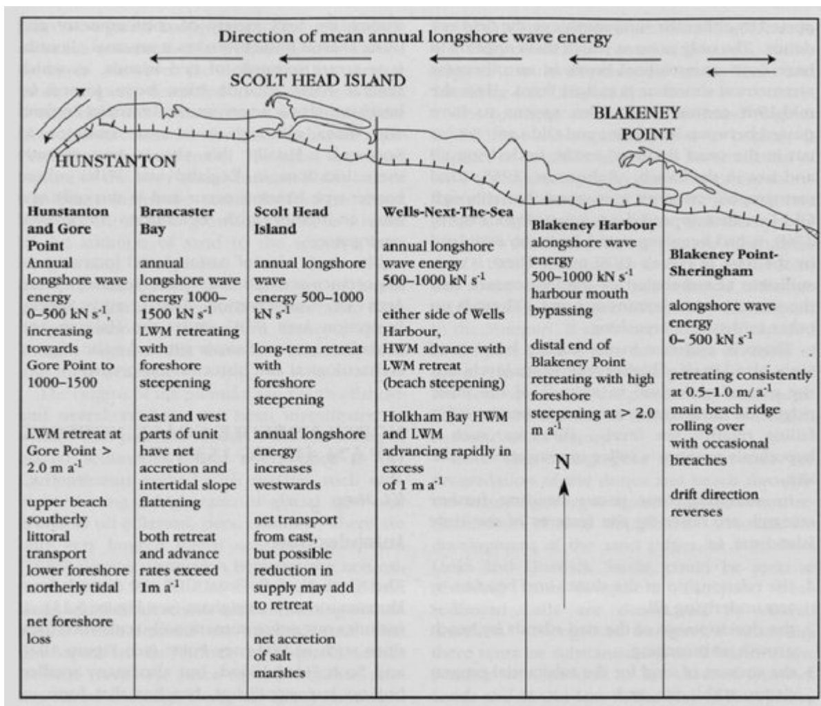
(Figure 11.27) Summary features and recent dynamics of the North Norfolk Coast GCR site from Hunstanton to Sheringham, and east to west distance of about 40 km. (After Halcrow, 1988.)
