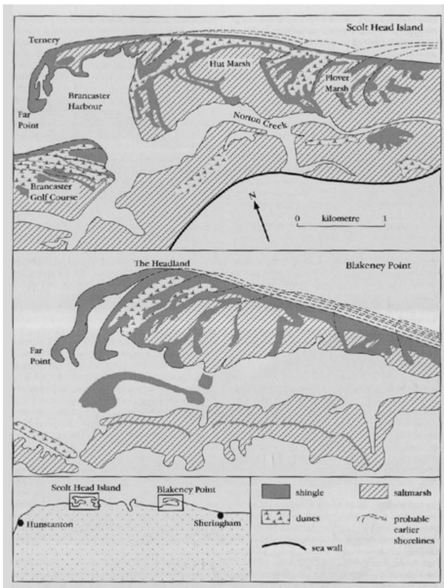
(Figure 11.30) (a) Scolt Head Island geomorphological features. (Based mainly on Steers, 1946b, 1960; Bird, 1984, 1985; Halcrow 1988.) (b) Blakeney Point geomorphological features. (Based mainly on Steers, 1946b; Bird, 1984, 1985; Flalcrow, 1988.)
