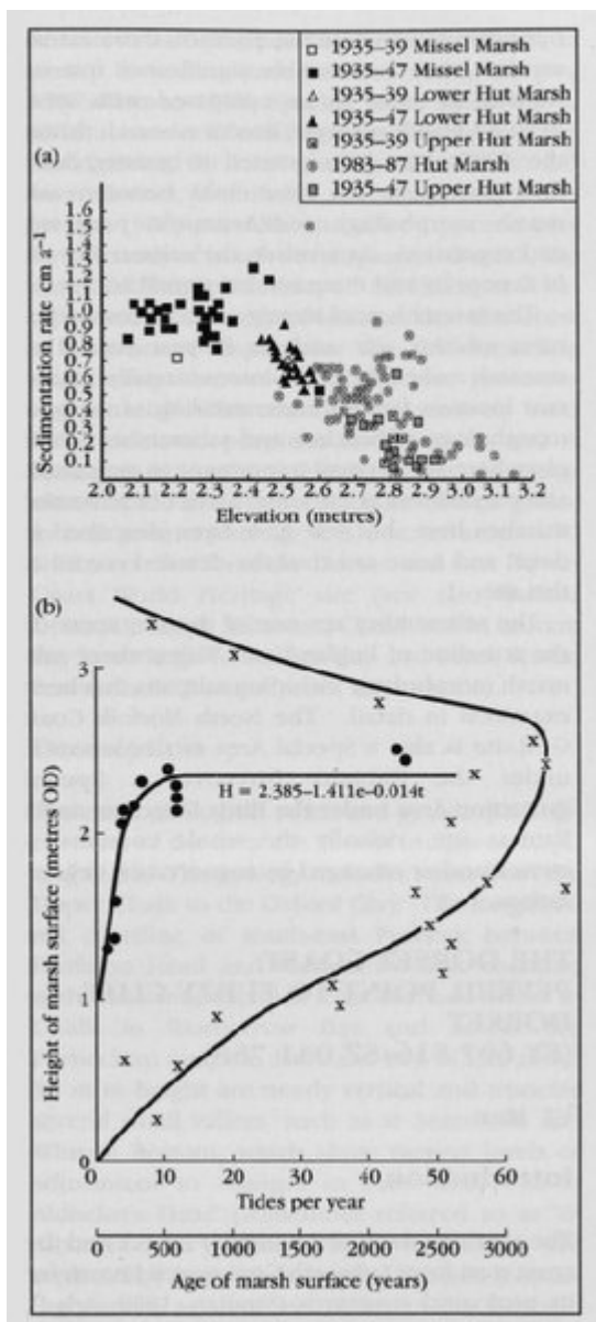
(Figure 11.31) Relationship of saltmarsh elevation to tides and age of the marsh surface at Missel Marsh, Lower Hut Marsh, upper Hut Marsh and Hut Marsh. H = 2.385 - 1.411 e^{-0.014t} is a best-fit line based on the relationship between marsh height ( H ), tides per year ( e ) and age of marsh surface ( t ). (After Pethick, 1980b; 1981.)
