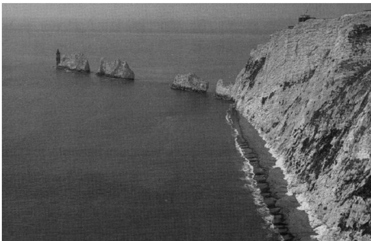
(Figure 4.16) The Needles and Scratchell's Bay, Isle of Wight, with narrow flint and chalk beach fed by contemporary rockfalls. (Photo: J.E. Gordon.)
