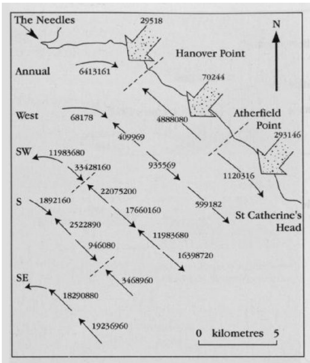
(Figure 4.17) Sediment inputs from cliff retreat ( m^3 a^{-1} ) annual longshore potential sediment transport and variations with wind direction. See text for explanation. Total sediment input = 392\,908\,m^3 a^{-1} (After Davies, 1997.)
