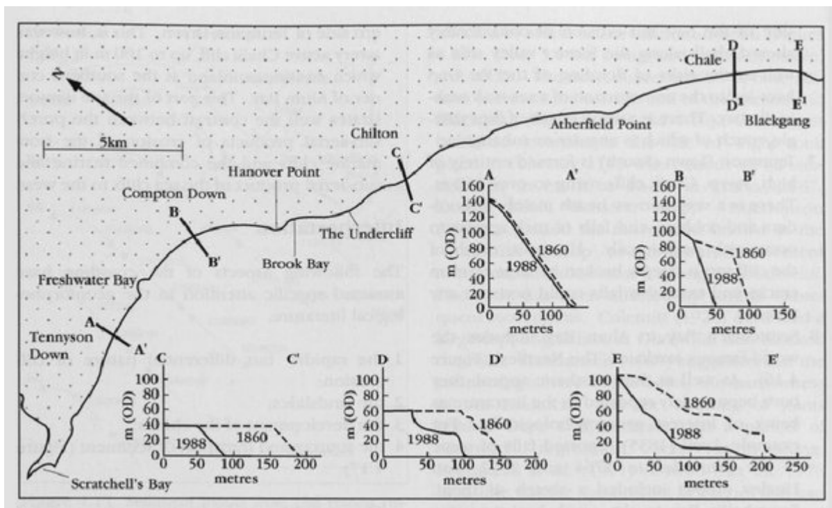
(Figure 4.15) Variations in the rates of cliff retreat from Blackgang to the Needles (to the west of Scratchell's Bay), Isle of Wight. Cliff profiles for sections A to E are shown. (After Hutchinson, 1984.)
