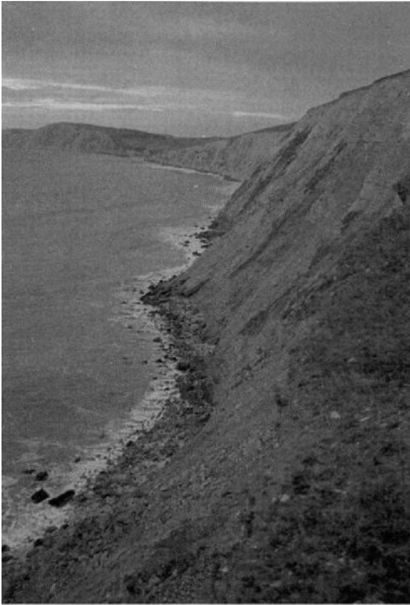
(Figure 4.19) Characteristic slope failures at Compton Down, looking west, showing shallow slides in chalk rock. (Photo: V.J. May.)
