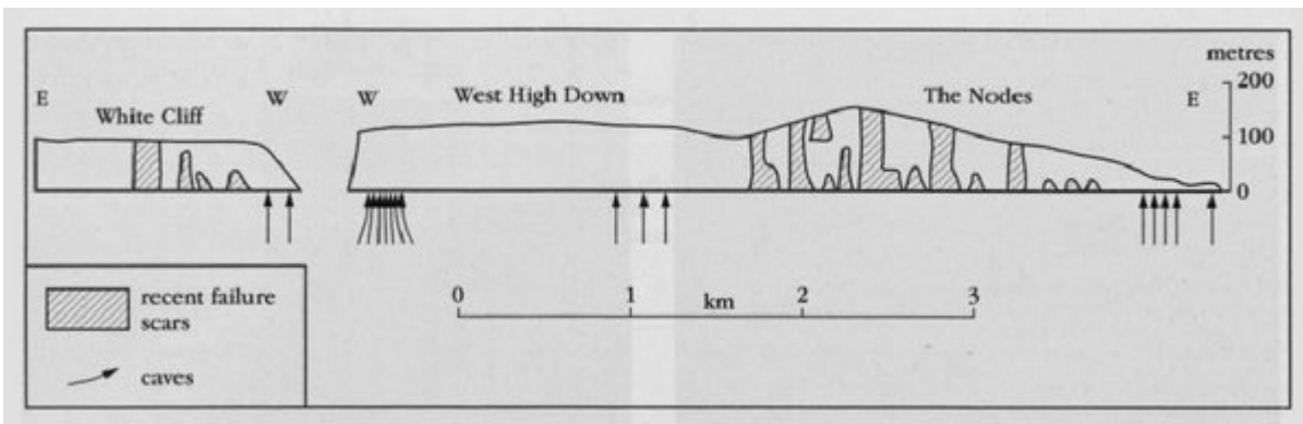
(Figure 4.21) Cliff-face failures west of Freshwater Bay. (Based on British Gas aerial survey, February 1996.)
