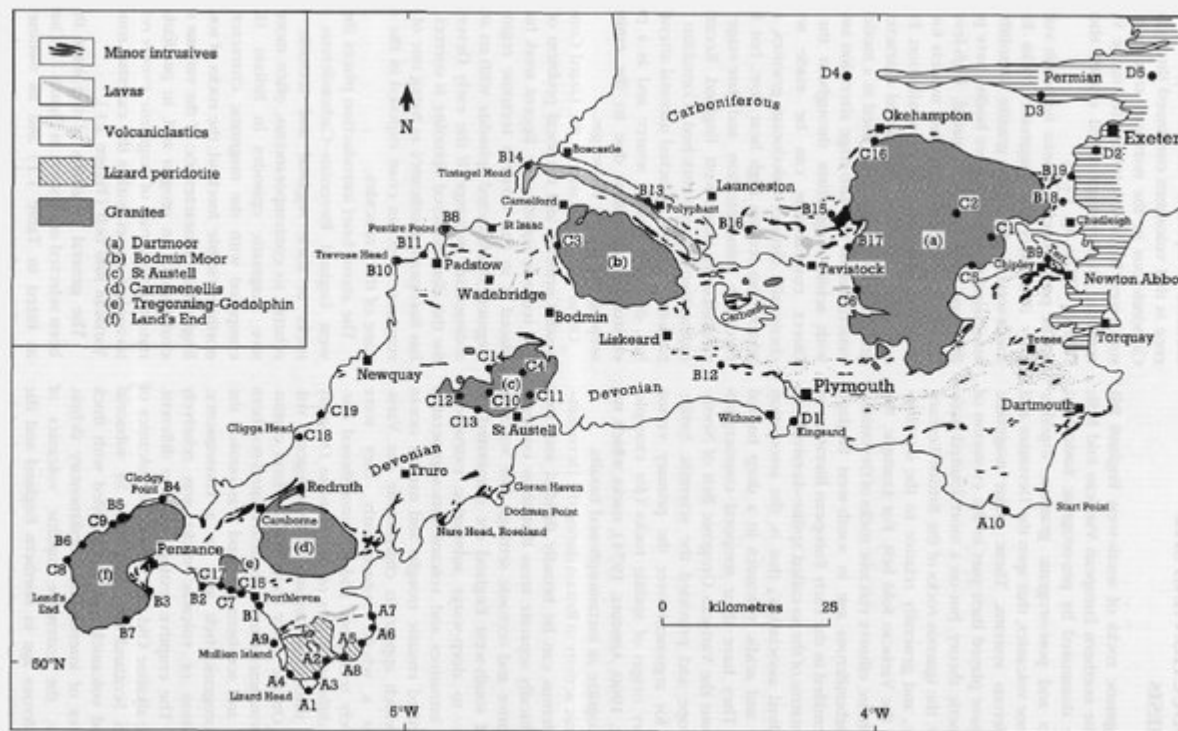
(Figure 1.1) Simplified geological map of south-west England showing the distribution of magmatic rocks and the approximate location of sites described in the text (modified from Floyd, 1982b). Sites are numbered and grouped as in (Table 1.1).
