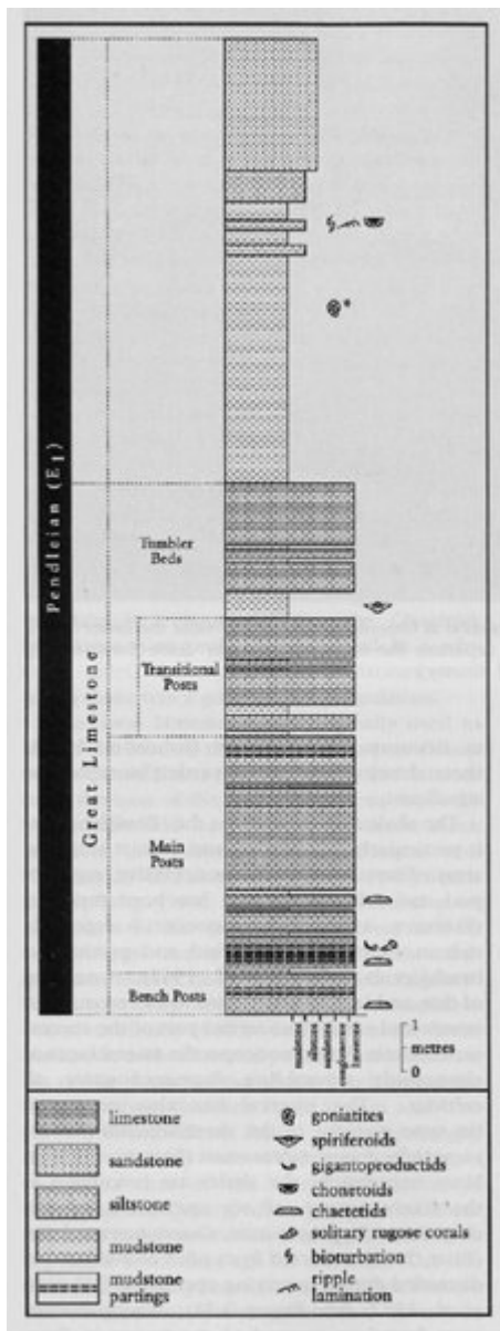
(Figure 3.23) Section of the Lower Namurian (Pendleian) Great Limestone succession at Greenleighton Quarry. An asterisk marks the position of a horizon of limestone nodules that Johnson et al. (1962) regarded as the most likely source of the basal E 1a goniatite marker Cravenoceras leion found in the tips nearby. Based on Johnson et al. (1962) and Fairbairn (1980).
