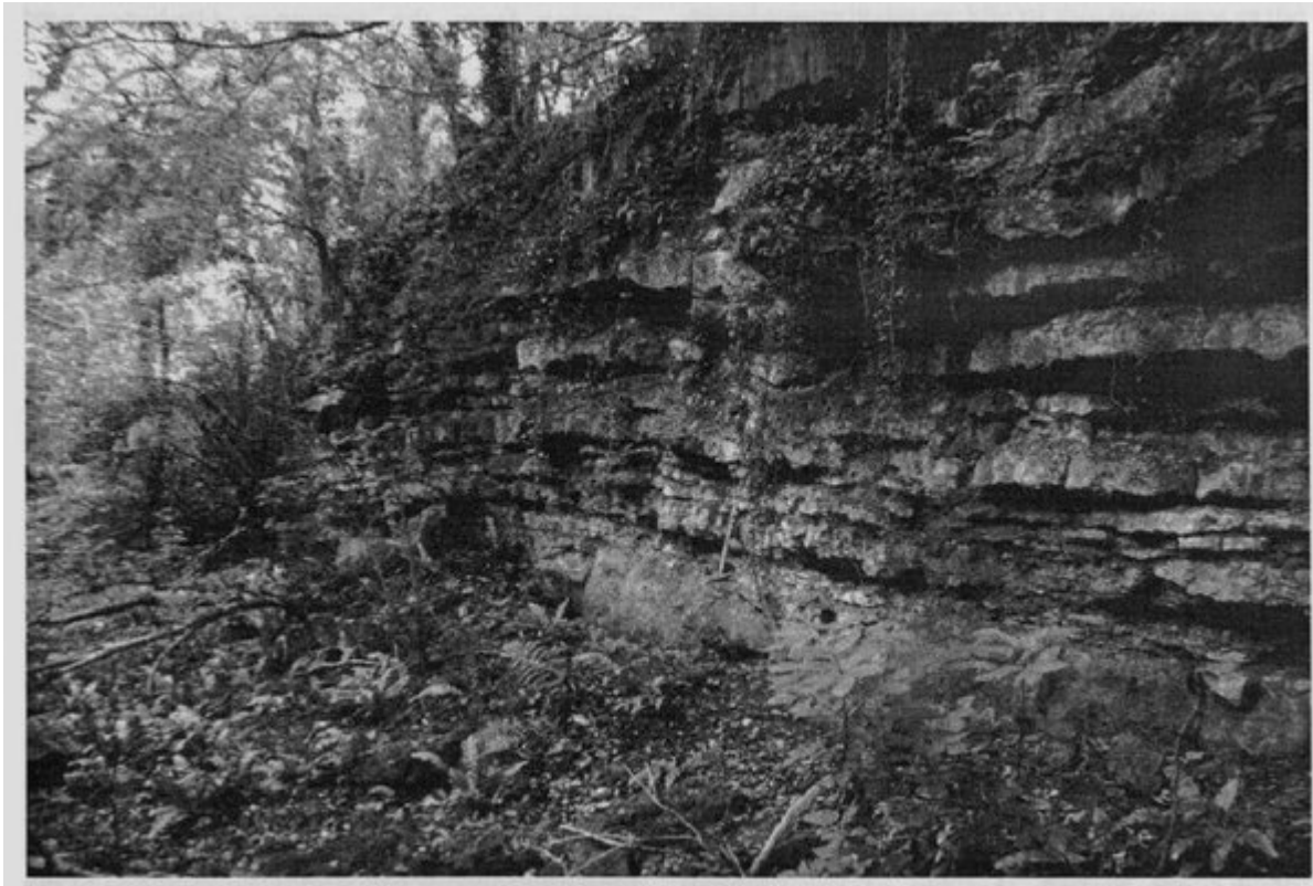
(Figure 7.35) Interbedded limestones and fissile mudstones in the lower unit of the Ticknall Limestone (Brigantian) at the Ticknall Quarries GCR site. The hammer towards the centre of the photograph indicates scale. (Photo: M.A. Purnell.)
