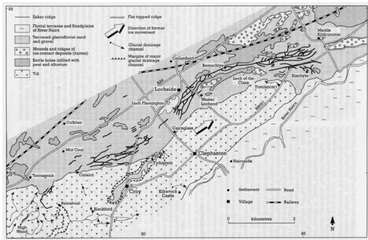
(Figure 7.11) Geomorphology of the Kildrummie Kames esker system between High Wood and Meikle Kildrummie (from mapping by C. A. Auton for the British Geological Survey 1:50,000 Geological Sheet 84W (Fortrose), in press).
