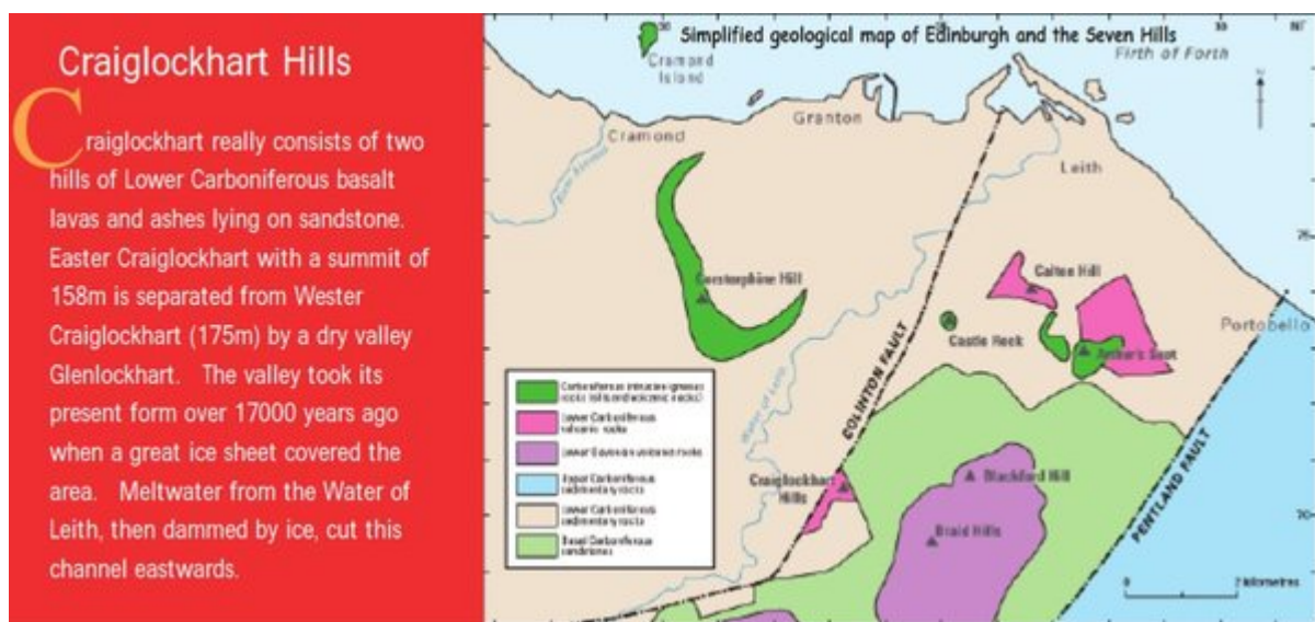
Simplified geological map of Edinburgh and the Seven Hills.
