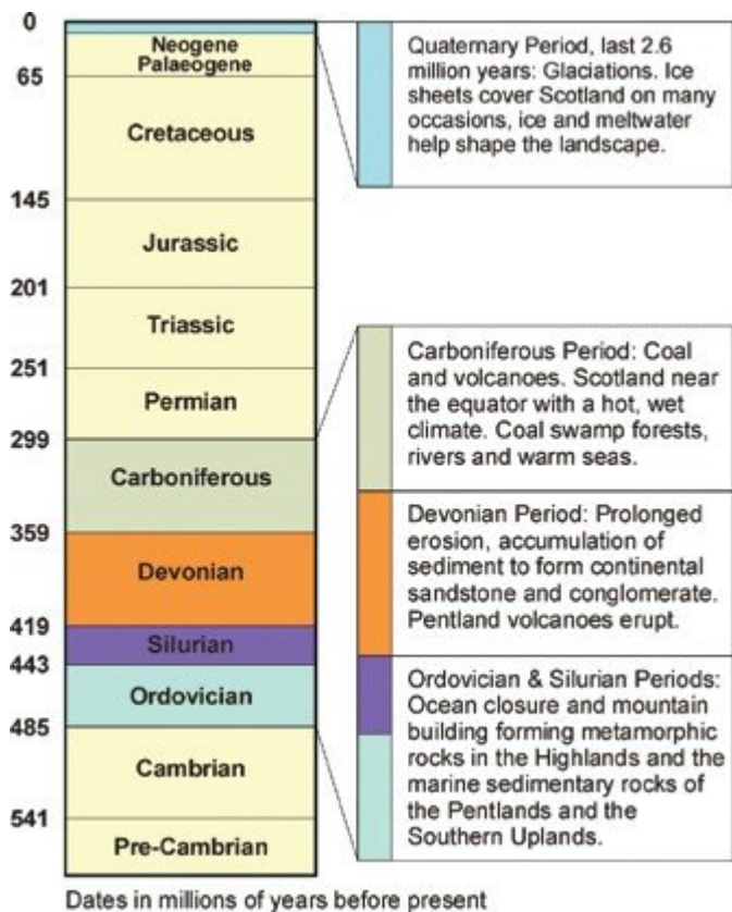
(Figure 3) Stratigraphic column
