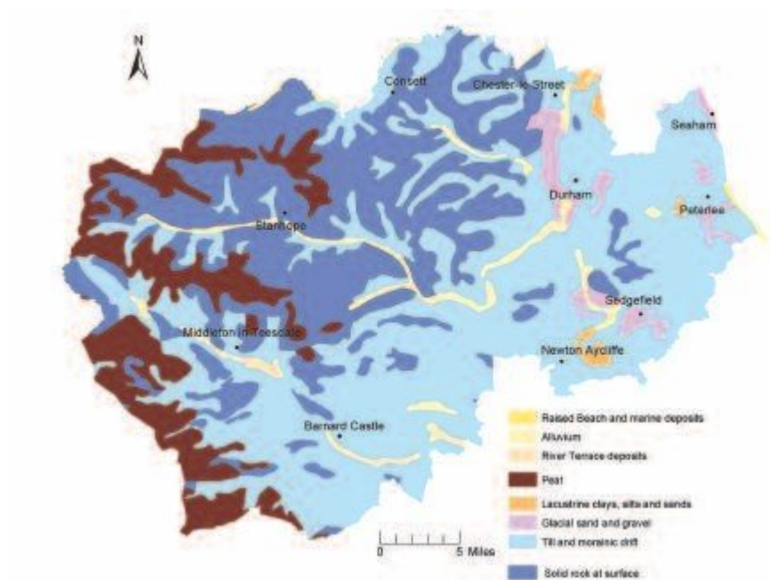
(Figure 24) Distribution of Quaternary deposits in County Durham .
