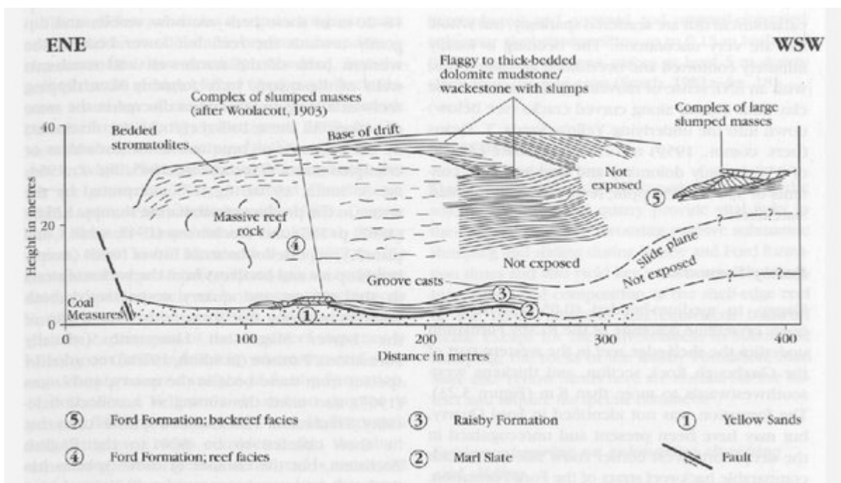
(Figure 3.22) Claxheugh Rock, Cutting and Ford Quarry, showing the position of the main features of geological interest.
