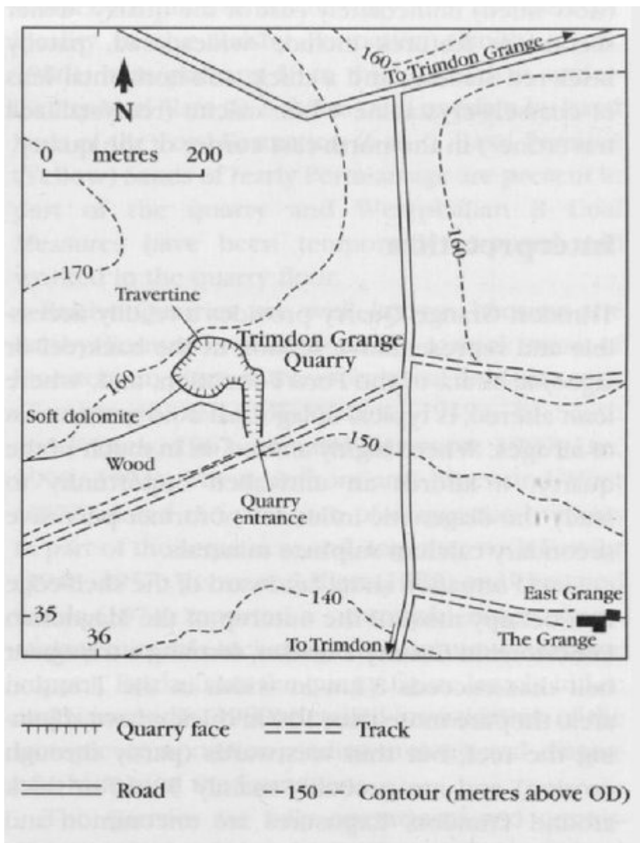
(Figure 3.60) Trimdon Grange Quarry and its immediate surroundings, showing the main features of geological interest.
