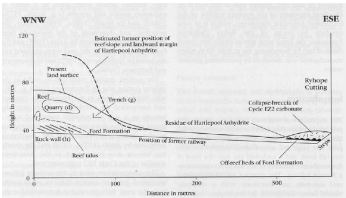
(Figure 3.34) Relationships of reef and off-reef (including post-reef) strata at the south-east end of Tunstall Hills and in the Ryhope Cutting (diagrammatic). See (Figure 3.31) for the location of the various exposures.
