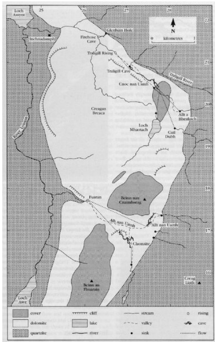
(Figure 8.2) Geological map of the main karst belt in Assynt, containing the caves of the Traigill and Allt nan Uamh Valleys. The dolomites belong to the Durness Group and are underlain by the Lower Palaeozoic quartzites. The cover rocks are klippe of Cambrian quartzite and Eocambrian sandstone lying over major thrust planes.
