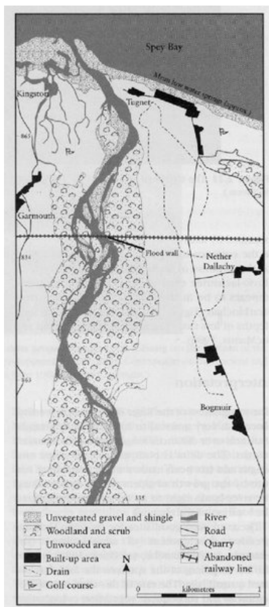
(Figure 2.22) The geomorphology of the Lower Spey.
